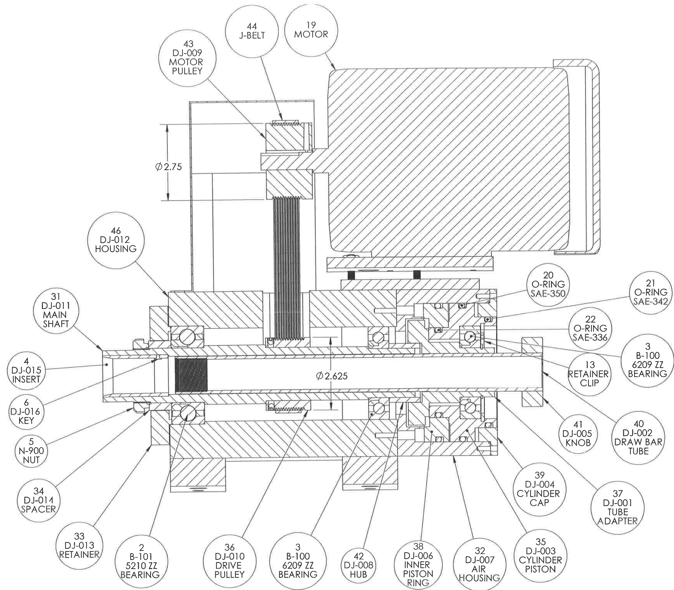
SECTION B-B
